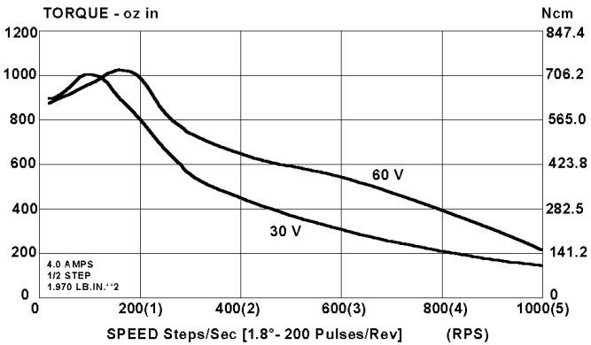
KML093F07 MOTOR, 4.0 Amp
