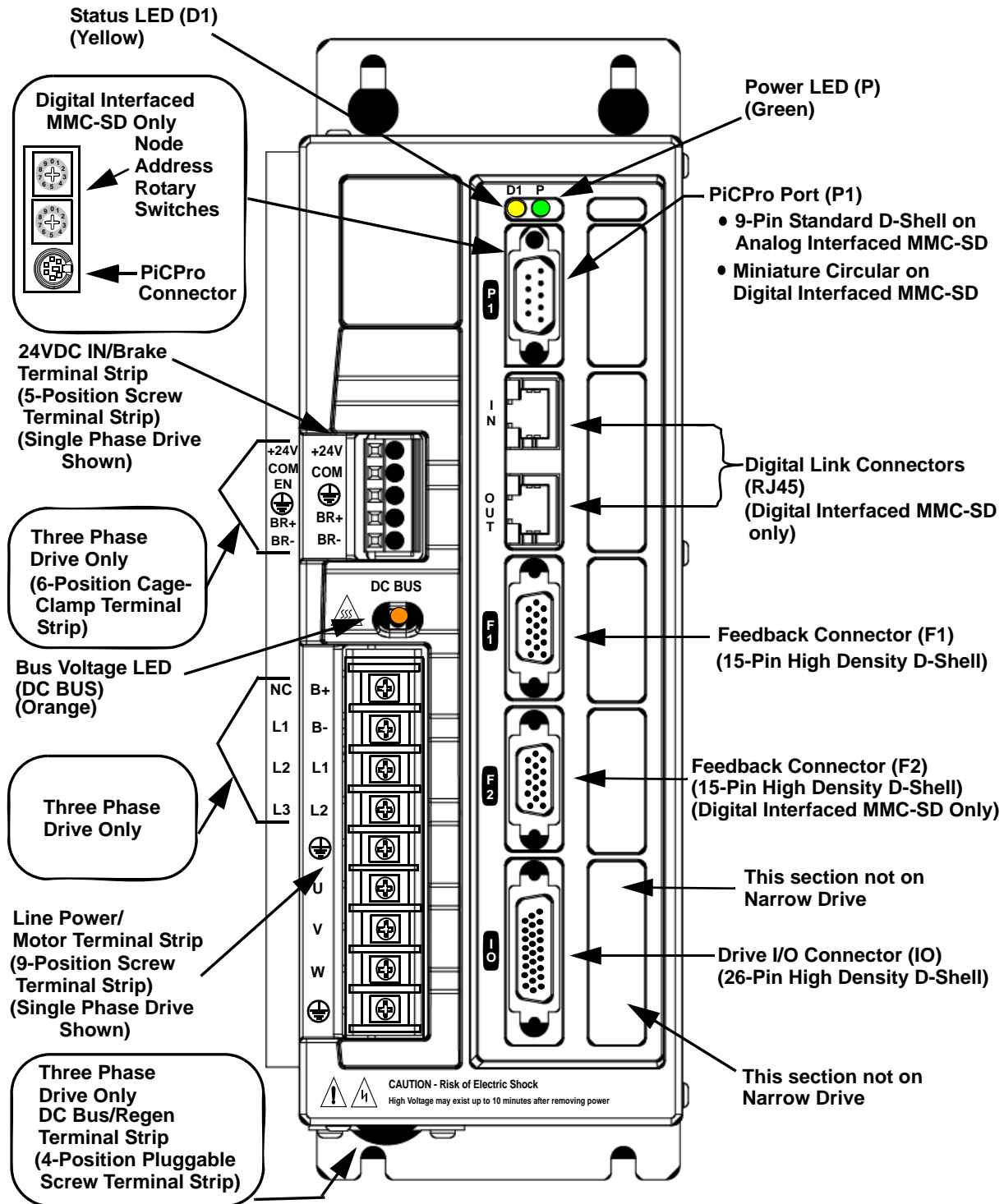
Figure 1-1: Front Panel, 230V Drives
