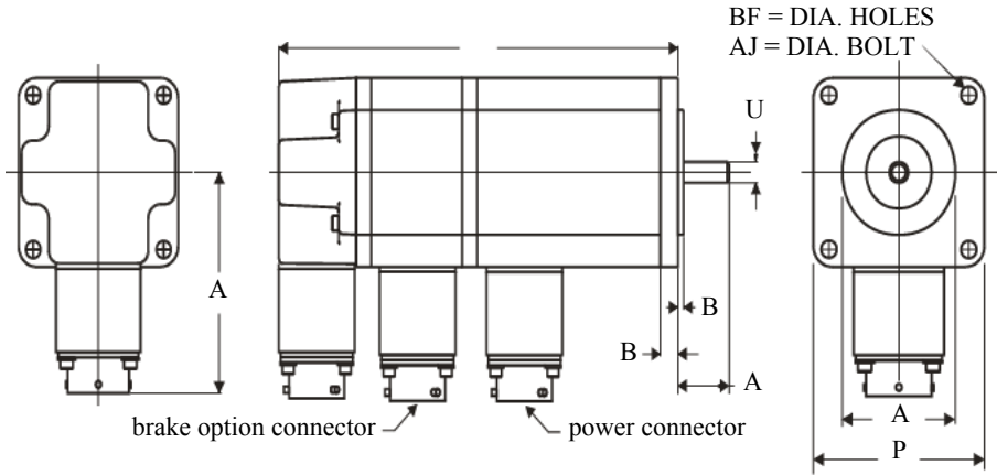
Figure 2 NSM34xx, NSM42xx, and NSM56xx Mounting Dimensions
