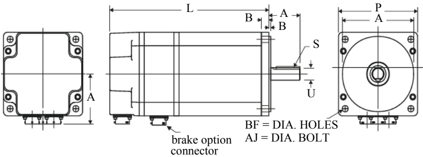
Figure 2 NSM34xx, NSM42xx, and NSM56xx Mounting Dimensions
