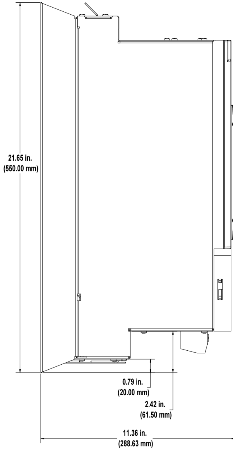
Figure 8-14: Size 3 460V Smart Drive - Side View
