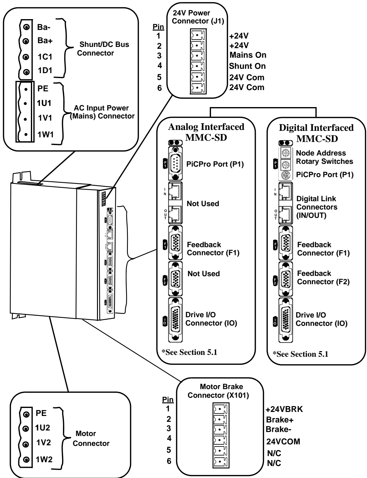
Figure 8-1: Connectors on the Size 1 460V Smart Drive
