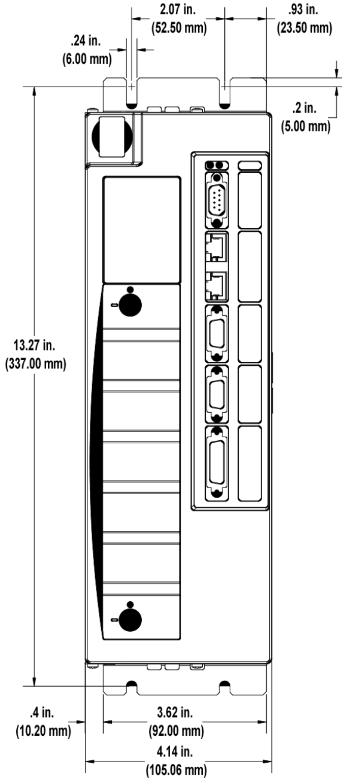
Figure 8-9: Size 1 460V Smart Drive - Front View
