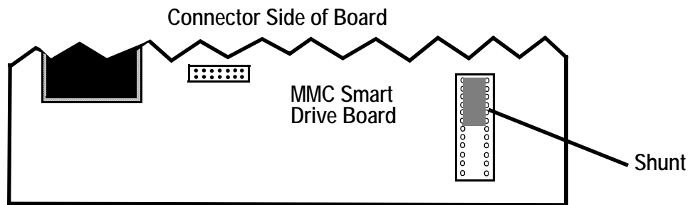
Figure 12-1: : Before Shunt Removed and Resolver Module Installed
