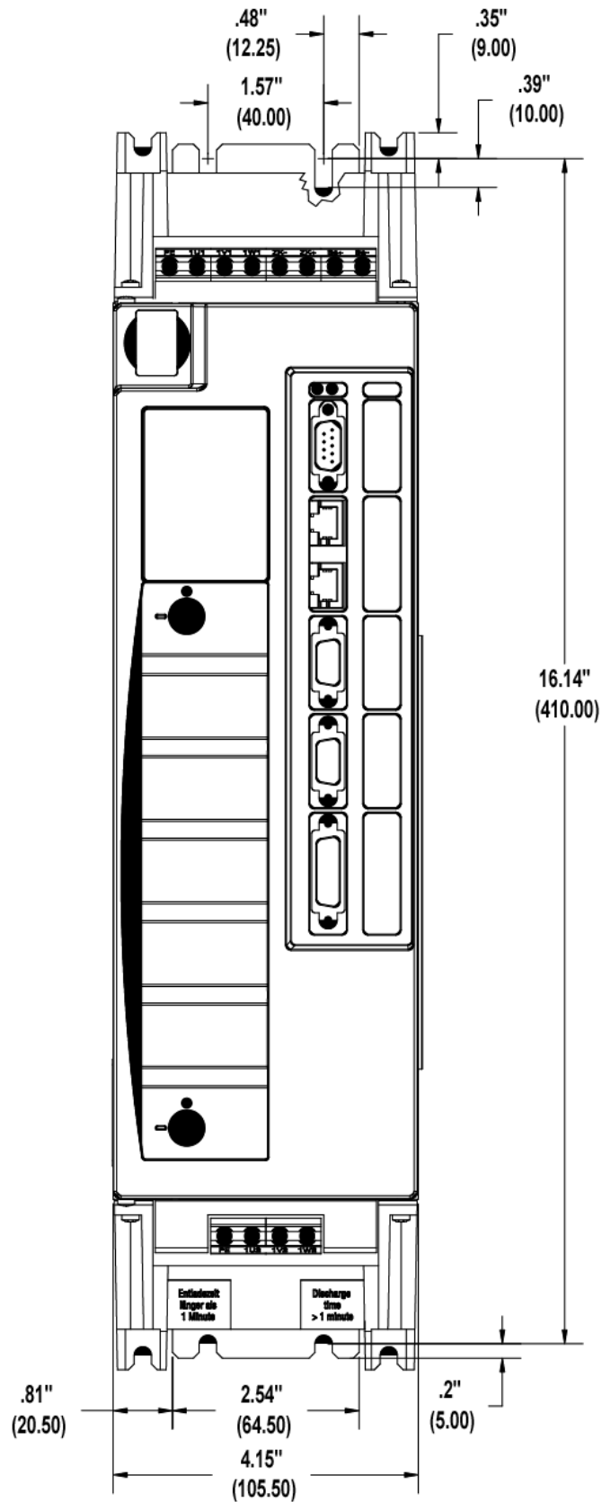
Figure 8-11: Size 2 460V Smart Drive - Front View
