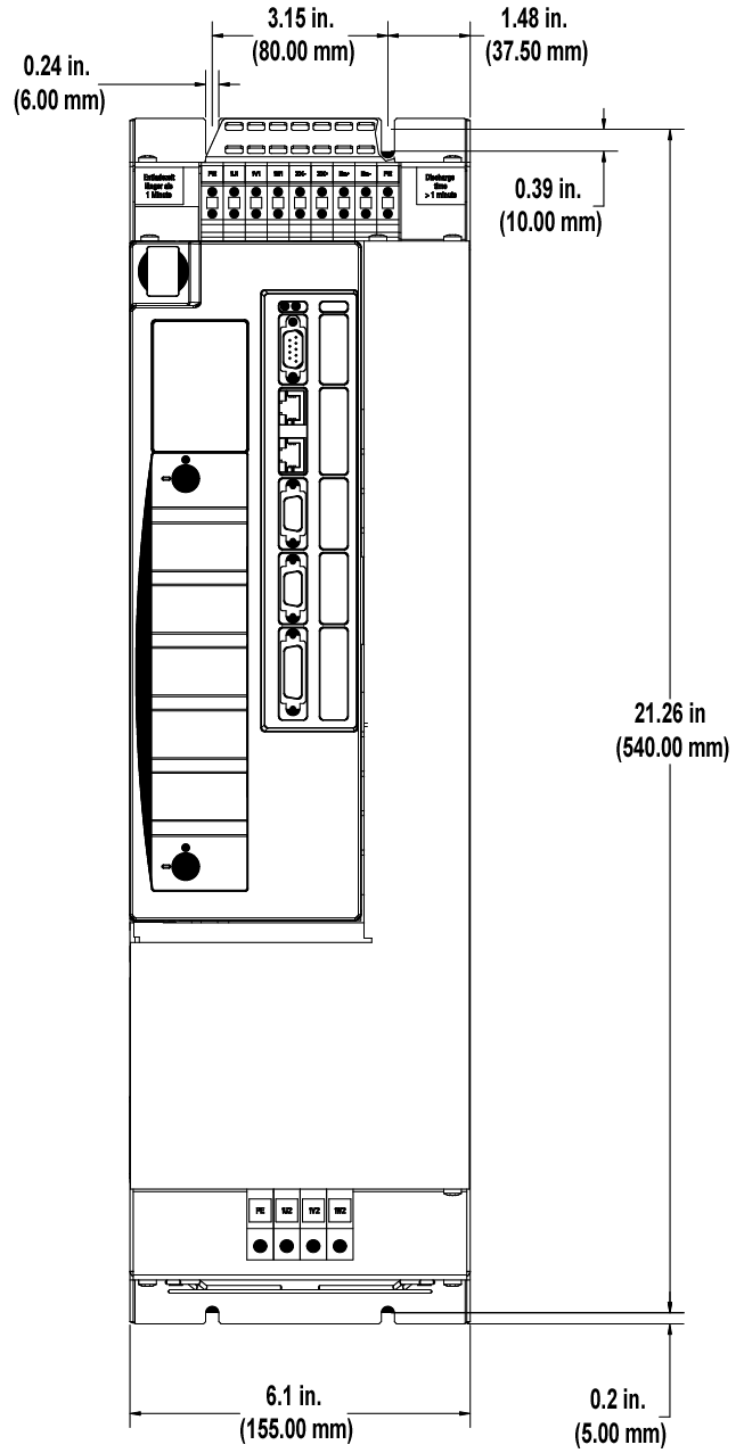
Figure 8-13: Size 3 460V Smart Drive - Front View
