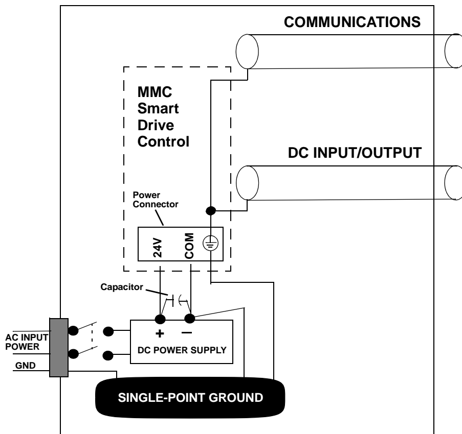
Figure 13-2: Recommended EMC Compliant Connections
