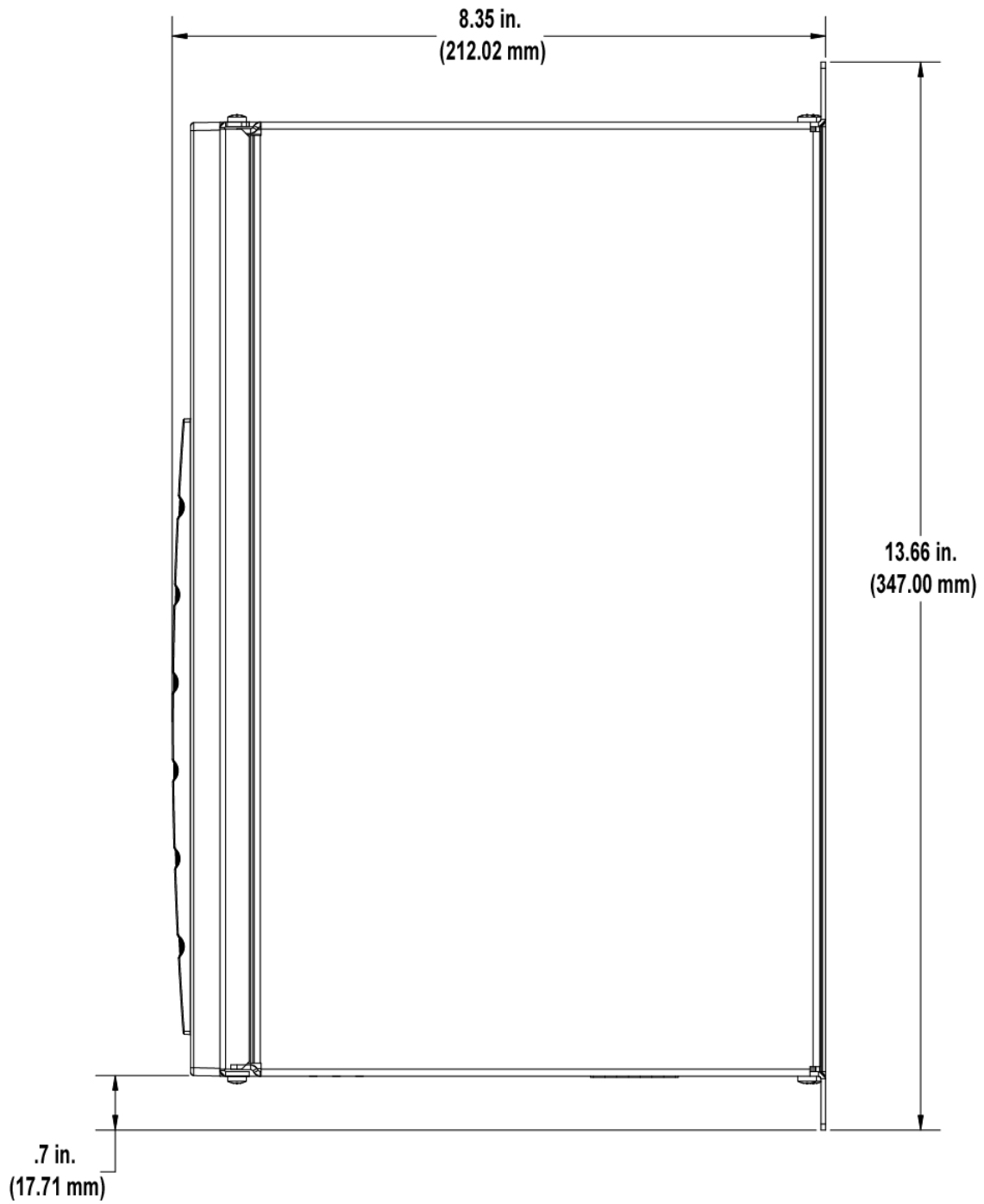
Figure 8-10: Size 1 460V Smart Drive - Side View
