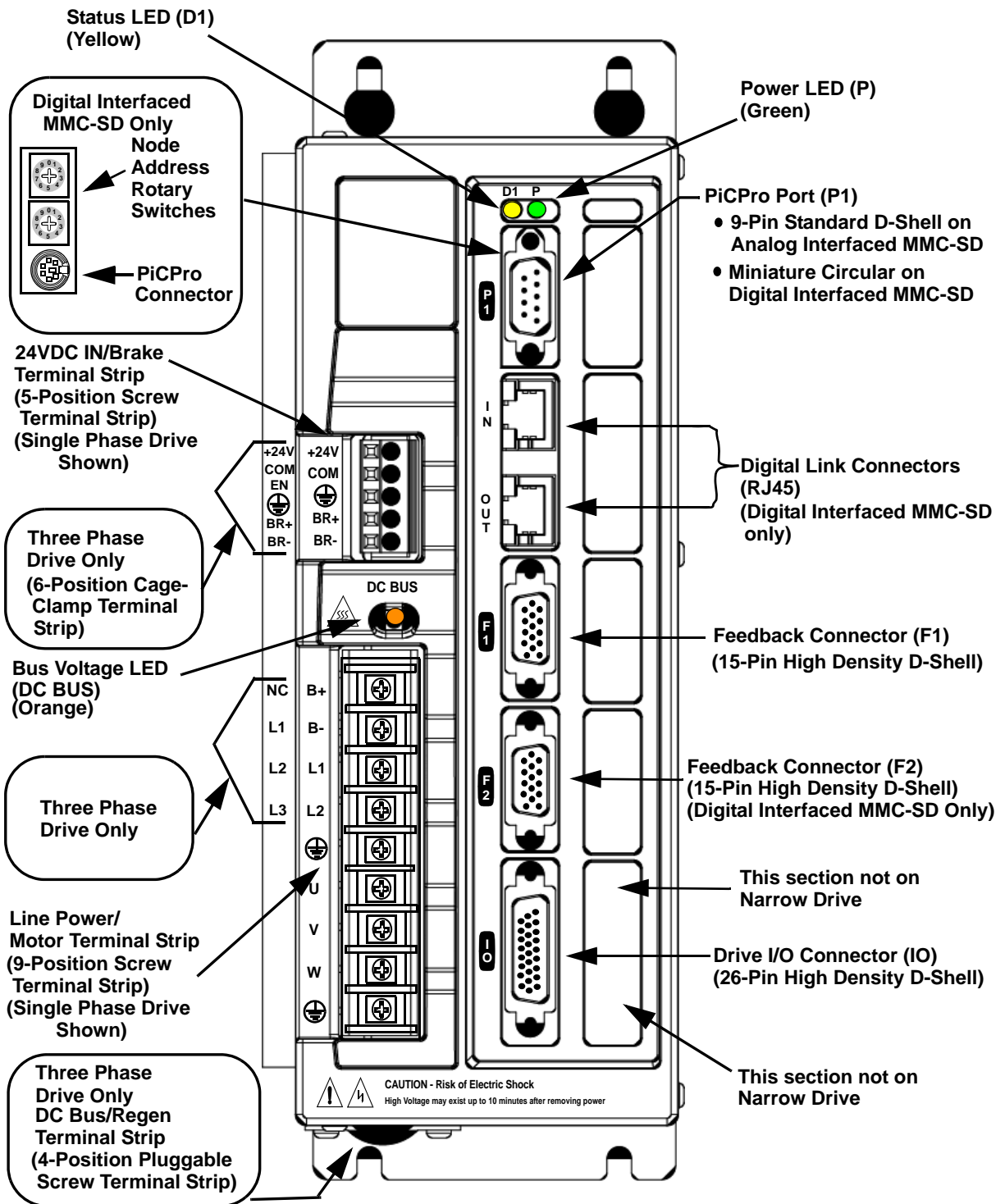
Figure 7-1: Front Panel, 230V Drives
