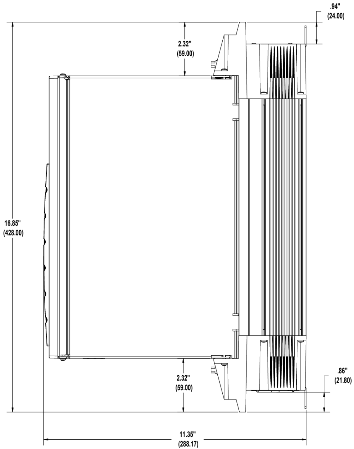
Figure 8-12: Size 2 460V Smart Drive - Side View
