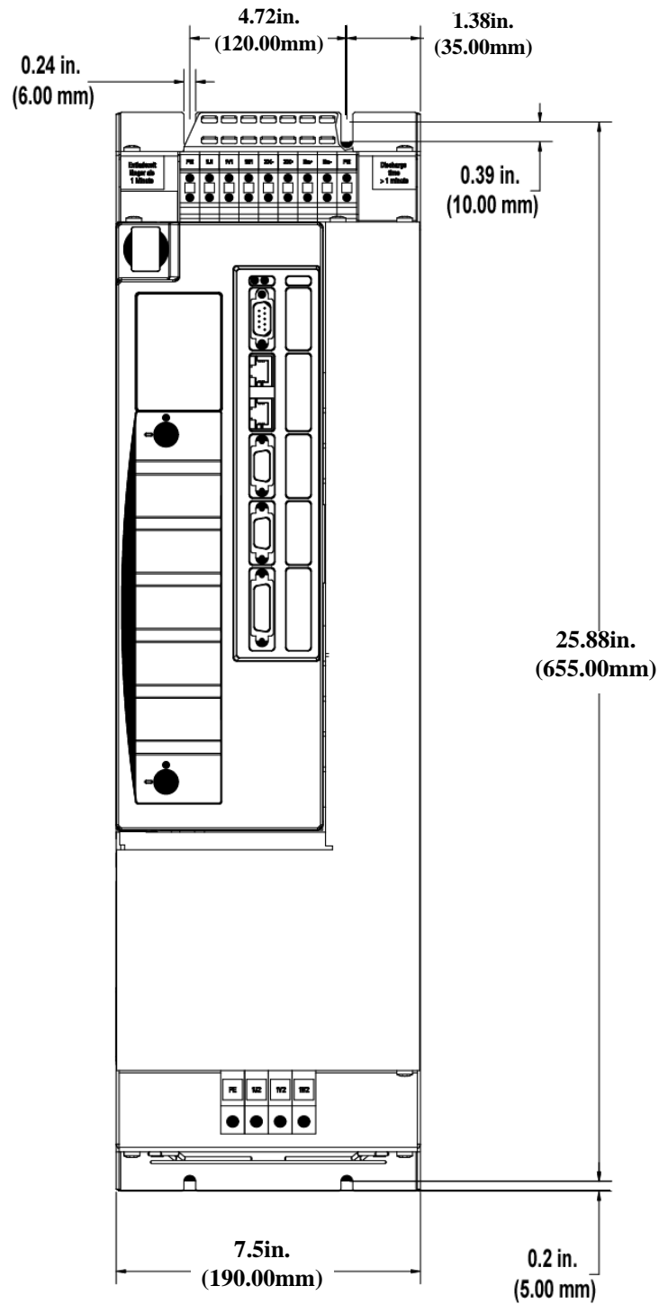
Figure 8-15: Size 4 460V Smart Drive - Front View
