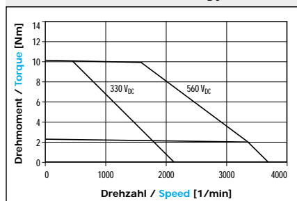
M406I 330/560 V DC
