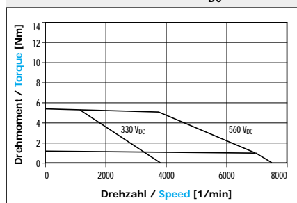
M404F 330/560 V DC
