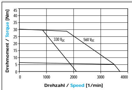
M506I 330/560 V DC
