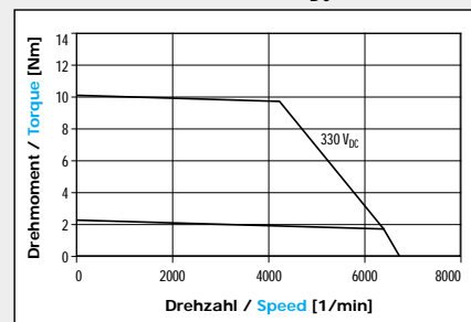
M406D 330 V DC
