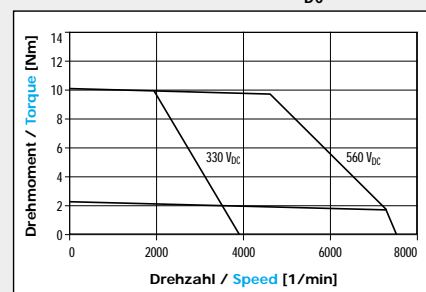
M406F 330/560 V DC
