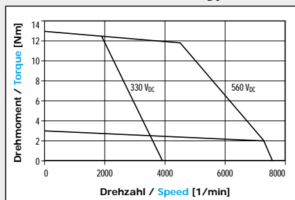
M408F 330/560 V DC
