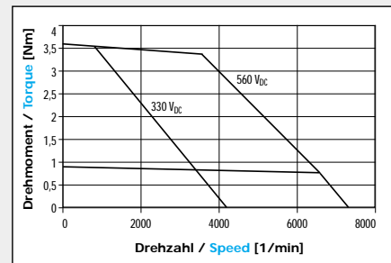
M258F 330/560 V DC
