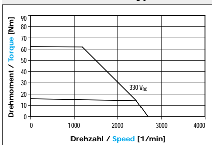
M714K 330 V DC
