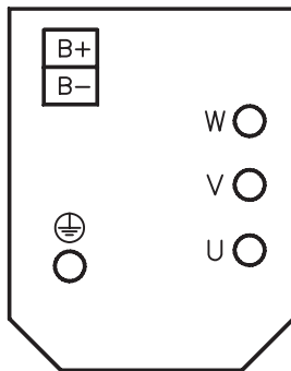
Connector ventilator
