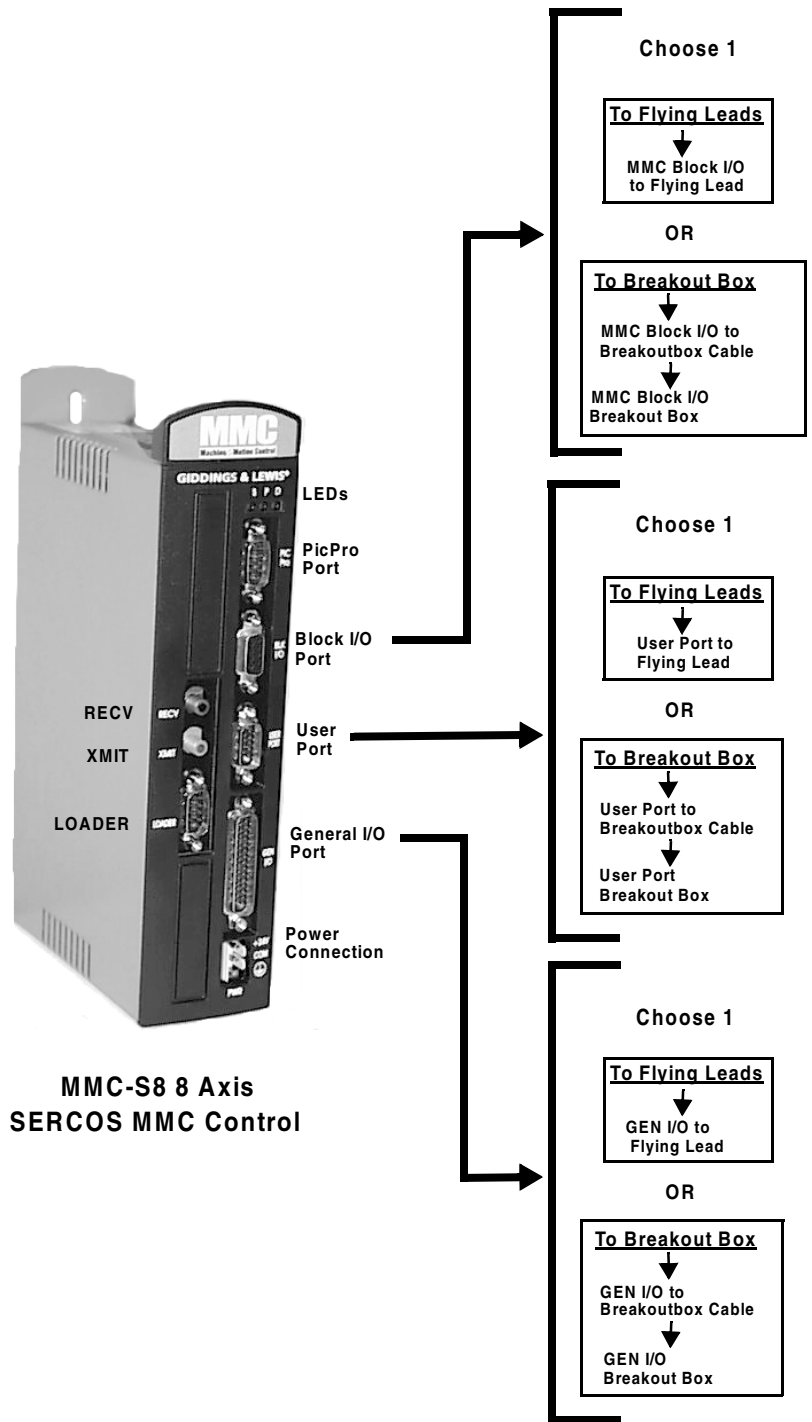
Figure C1-2: Connection Selector Sheet for MMC SERCOS Control
