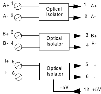
Figure C1-7: Connections from Encoder to Encoder Isolated AUX I/O
