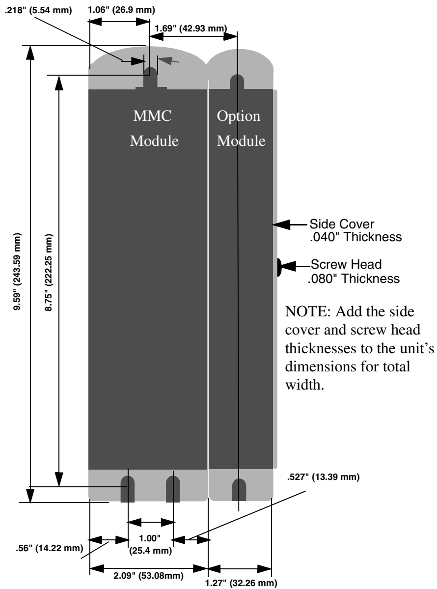
Figure 5: MMC Mounting Dimensions with Option Module Attached
