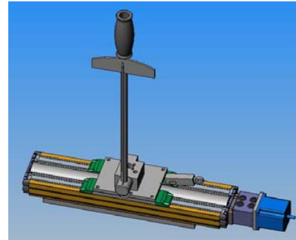
PITCH MEASURING SET UP
